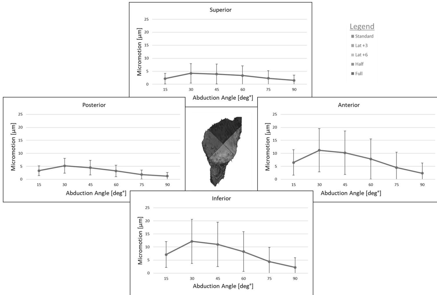
Figure 3-5 – Maximum normal micromotion [μm] for various abduction angle [deg°], by quadrant of the glenoid (mean±SD)
