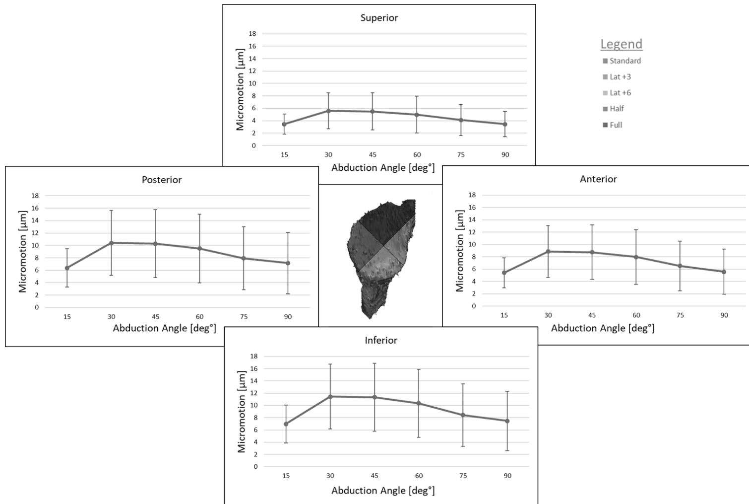
Figure 3-7 – Maximum tangential micromotion [ \mu\text{m} ] for various abduction angles [ \text{deg}^\circ ], by quadrant of the glenoid (mean \pm SD)
