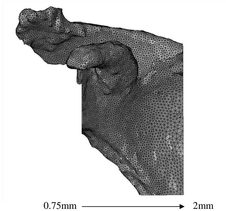
Figure A-2 – Mesh element size increasing from 0.75mm (left) to 2mm (right)
